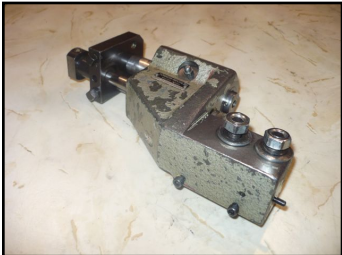
Broaching toolholder Ref : 108649 - AS32/4 AS14 - SAS16 - SAS16.6
