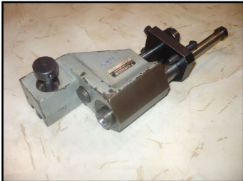
Broaching toolholder Ref : 107625 - AS32/5-1 AS14 - SAS16 - SAS16.6
